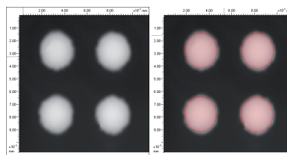
Automatic detection of BGA bumps
